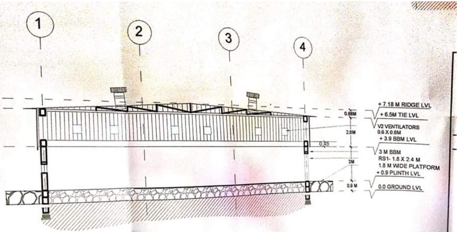
SECTION BB' SCALE - 1:75
