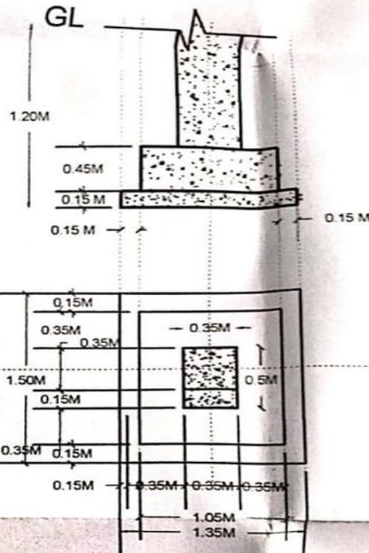
C1 COLUMN FOOTING. C2 & C3 COLUMN FOOTING.
