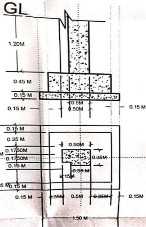
C1 COLUMN FOOTING. C2 & C3 COLUMN FOOTING.
